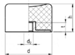
TYPE GBSE
